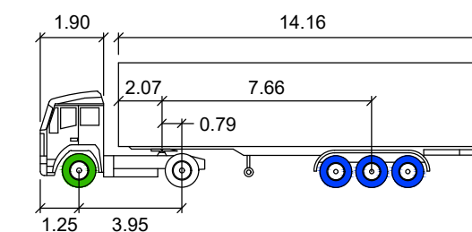
Sattelschlepper Rm=7.5m
